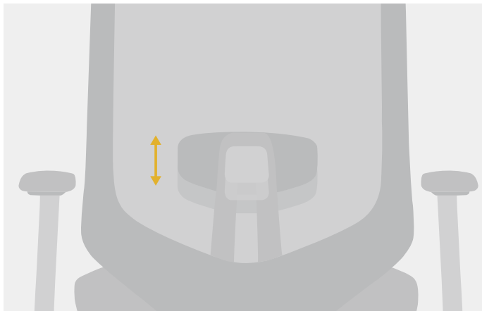
Waist up and down adjustment, Adjusting distance 70 mm
